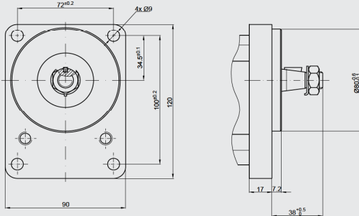
T Square flange centering \varnothing 80 mm
