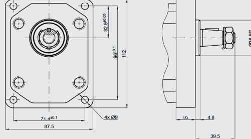
W SAE J 744 82-2 A \varnothing 82.55 mm
