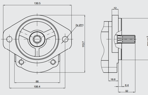
W SAE J 744 82-2 A \varnothing 82.55 mm
