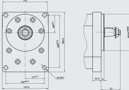
V Square flange centering \varnothing 105 mm
