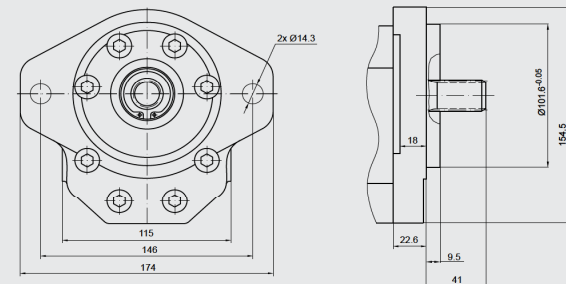
X SAE J 744 101-2 B \varnothing 101.6 mm
